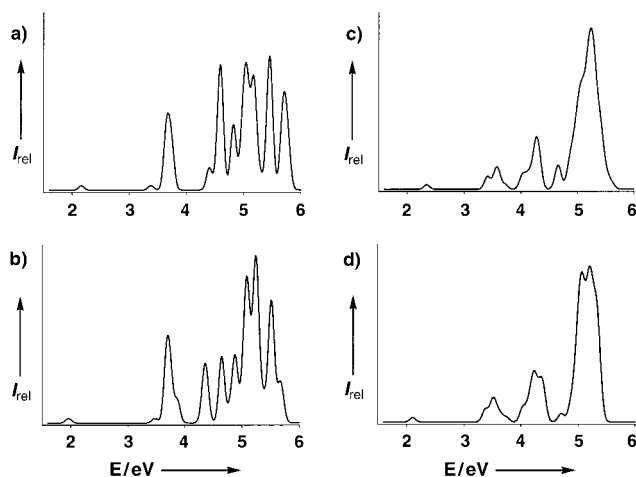
Figure 4. The simulated photoelectron spectra of MoAu 12 - and WAu 12 - . a) I h MoAu 12 - , b) I h WAu 12 - , c) O h MoAu 12 - , and d) O h WAu 12 - .
