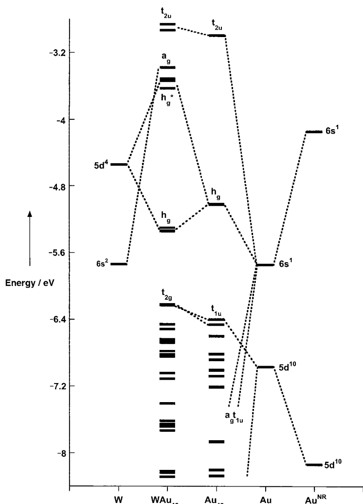
Figure 3. The energy-level correlation diagrams of W, Au, Au 12 , and I h W@Au 12 . All of the energies are calculated at the scalar-relativistic level, except for Au NR which is calculated at the non-relativistic level. The HOMO ( h g ) and LUMO ( h g * ) of the I h W@Au 12 are indicated.
